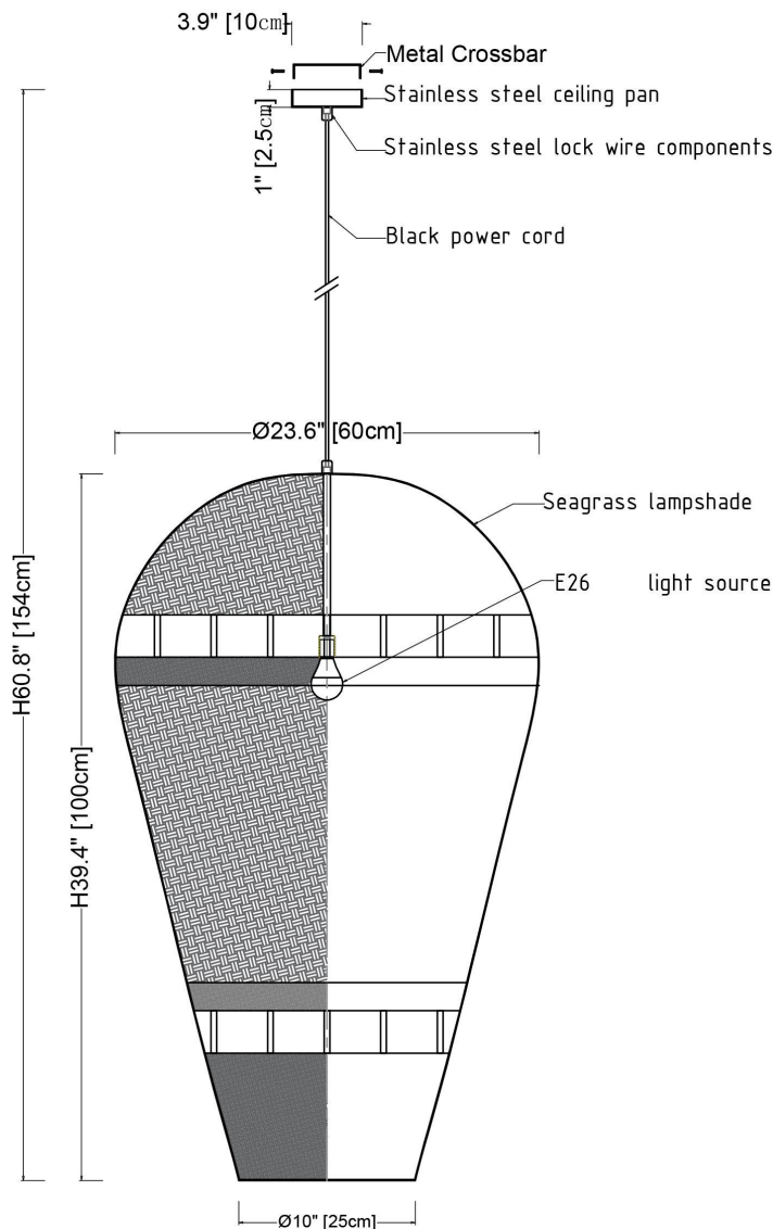
Front view
